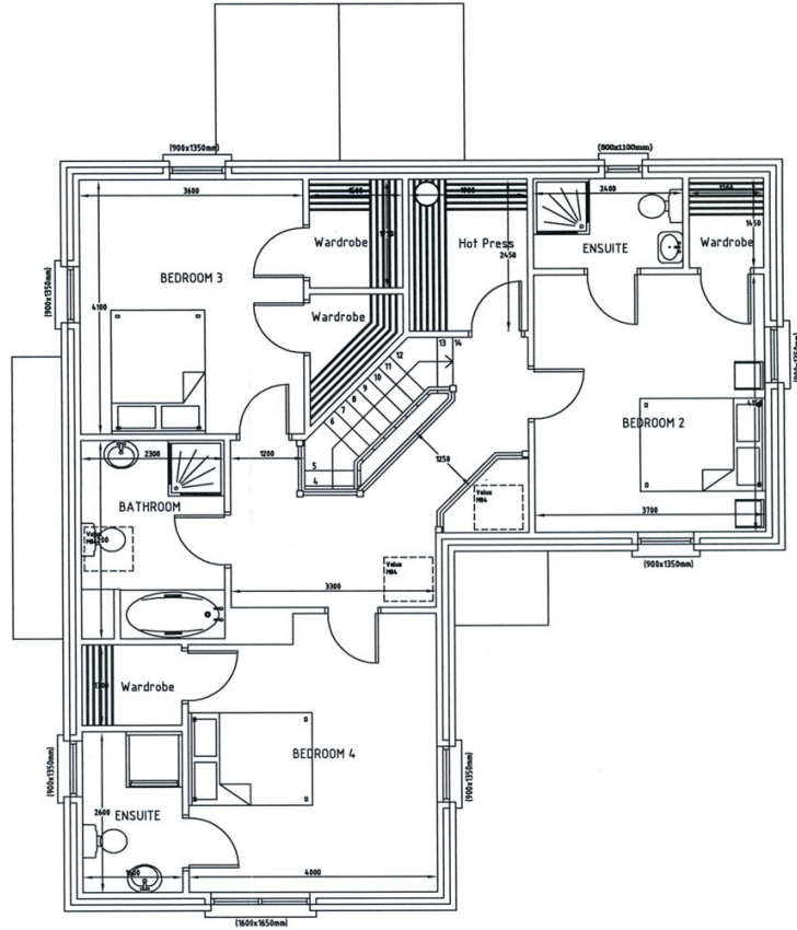
FIRST FLOOR LAYOUT PLAN
