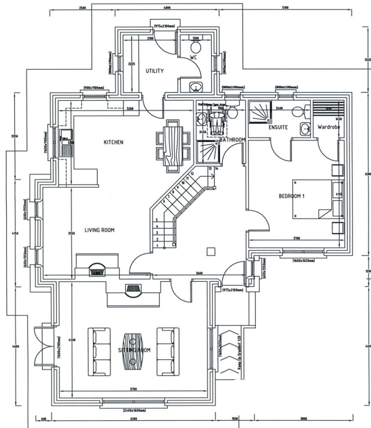
GROUND FLOOR LAYOUT PLAN
